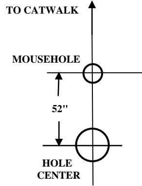
TYPICAL RIG LAYOUT
