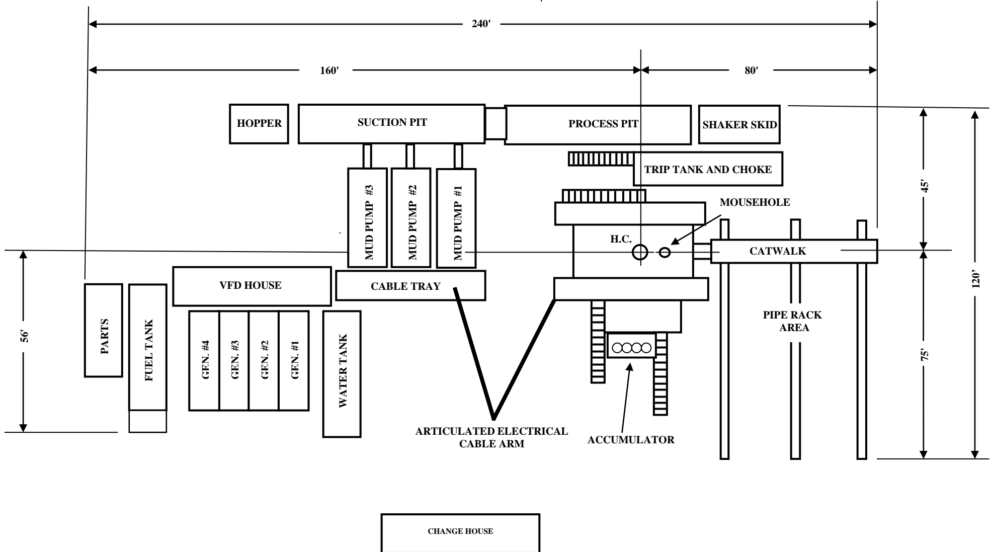
TYPICAL RIG LAYOUT
